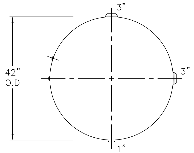
VIEW W/O SUPPORTS
