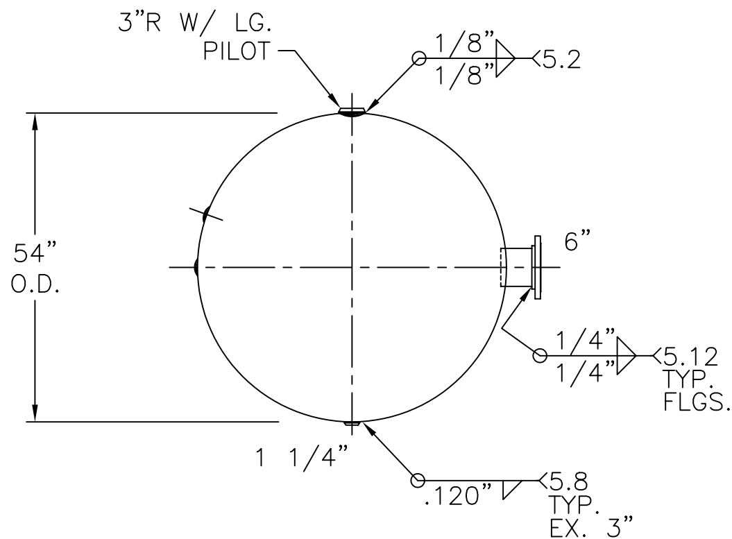
END VIEW W/O SUPPORTS
