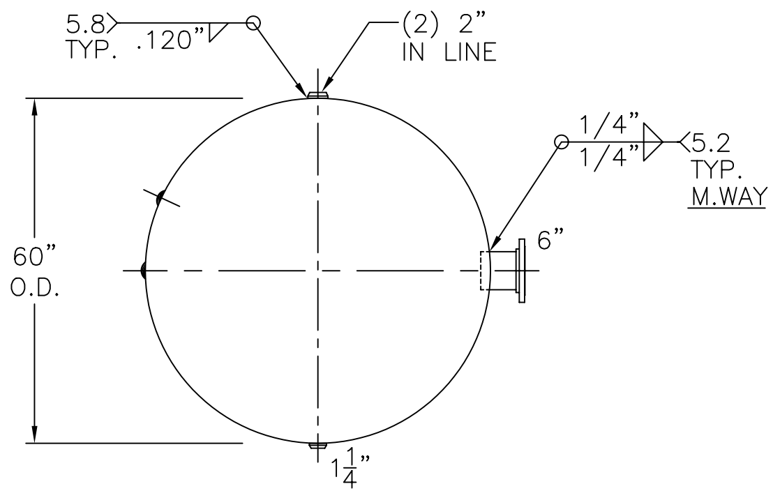
END VIEW W/OUT SUPT'S
