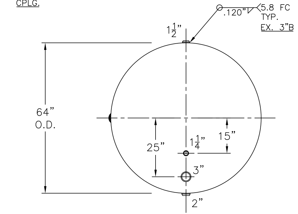
VIEW W/OUT SUPPORTS
